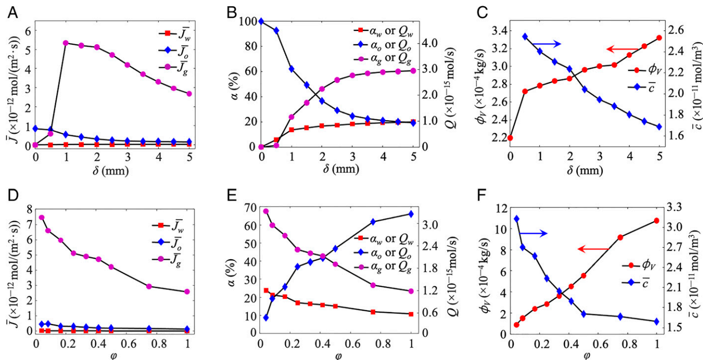
Fig. 4. The influence of the gap thickness \delta and the opening size \phi on: (A, D) the average smoke flux on the water, opening and gap surfaces, (B, E) the absorption rate of smoke on the water surface, and leakage rates through the opening and the gap, as well as their proportions, and (C, F) the ventilation rate and the average smoke concentration in the lamp. The opening size is 1/4 for (A-C). The gap size is 2 mm for (D-F).
